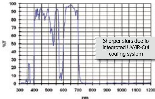
Spectral Transmission NEODYMIUM Moon & Skyglow Filter
